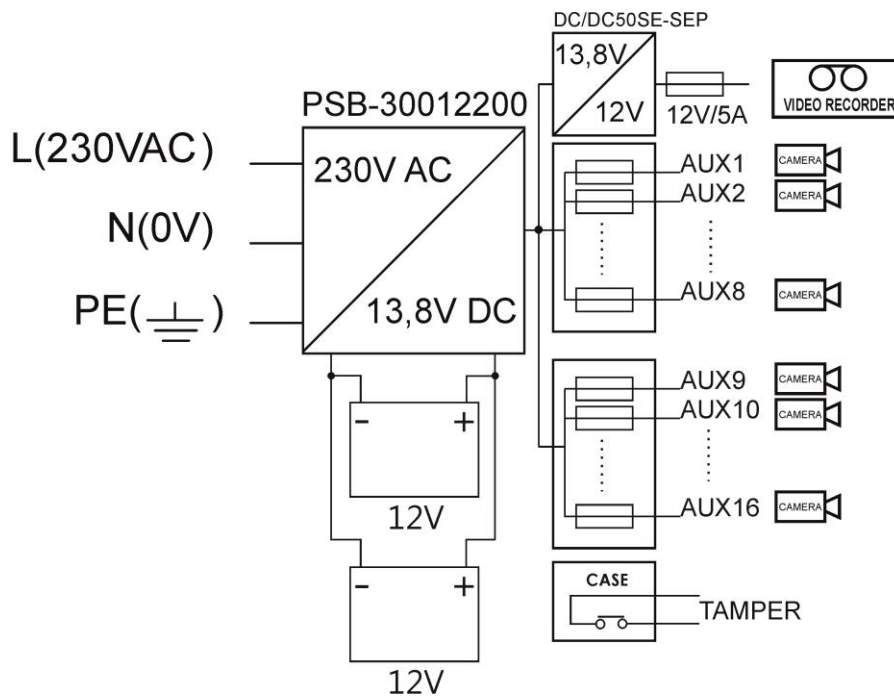
Fig.1. Block diagram of the PSU.
