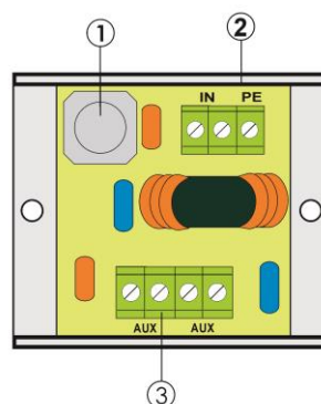
Fig.3. Output filter.
